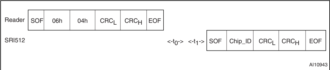
Figure 53. Pcall16 frame exchange between reader and SRI512
